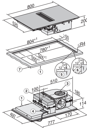
KMDA7272FL, KMDA7473FL – flush – Installation drawing
